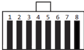
RJ-45/RJ-48/RJ-61 - 8P8C
