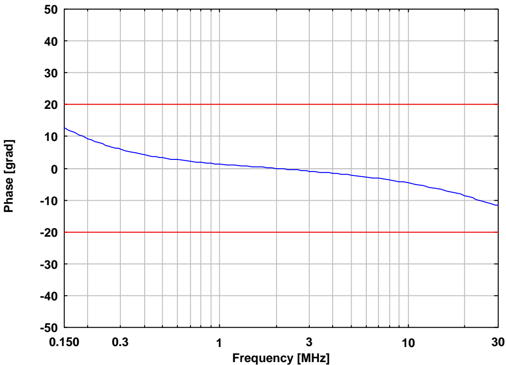
Abb. 7 Common Mode Impedance (Phase) at EuT-Terminals
