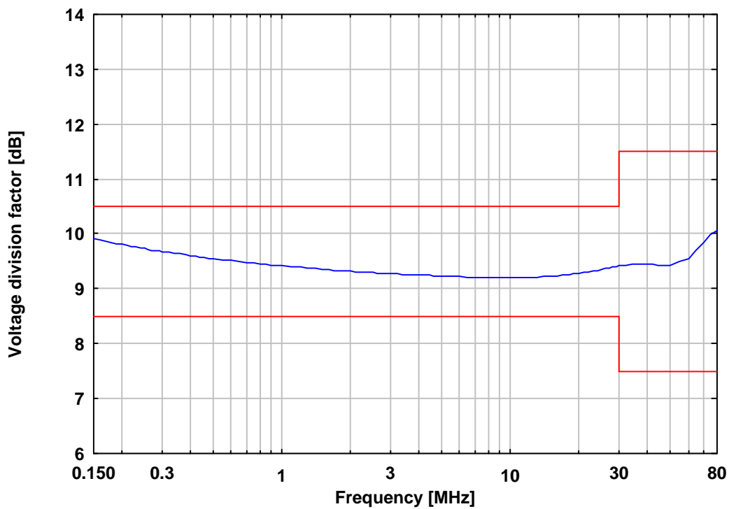
Abb. 5 Transmission EuT to Measurement Port
