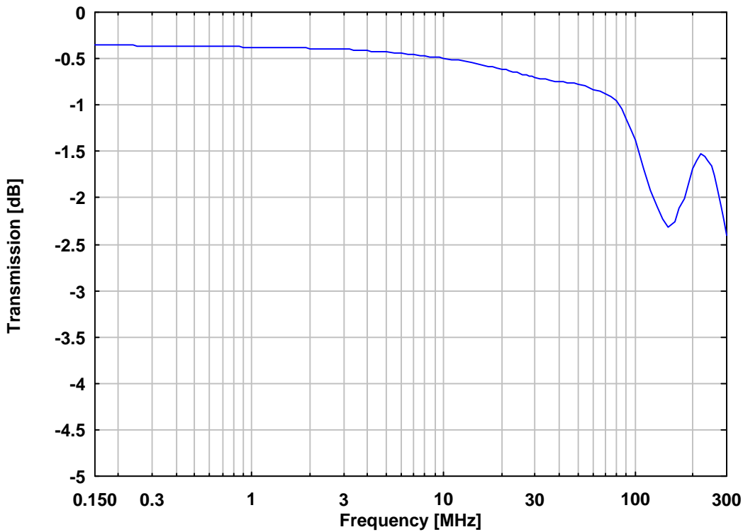
Abb. 2 Transmission Differential Mode Signal AE-EuT
