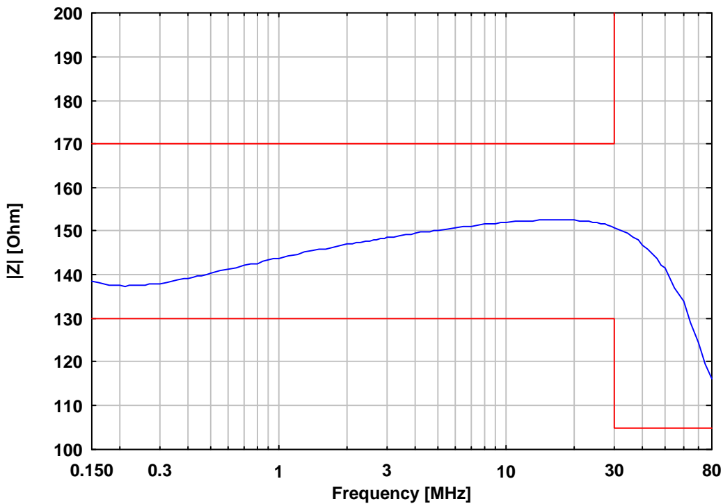
Abb. 6 Common Mode Impedance (Magnitude) at EuT-Terminals
